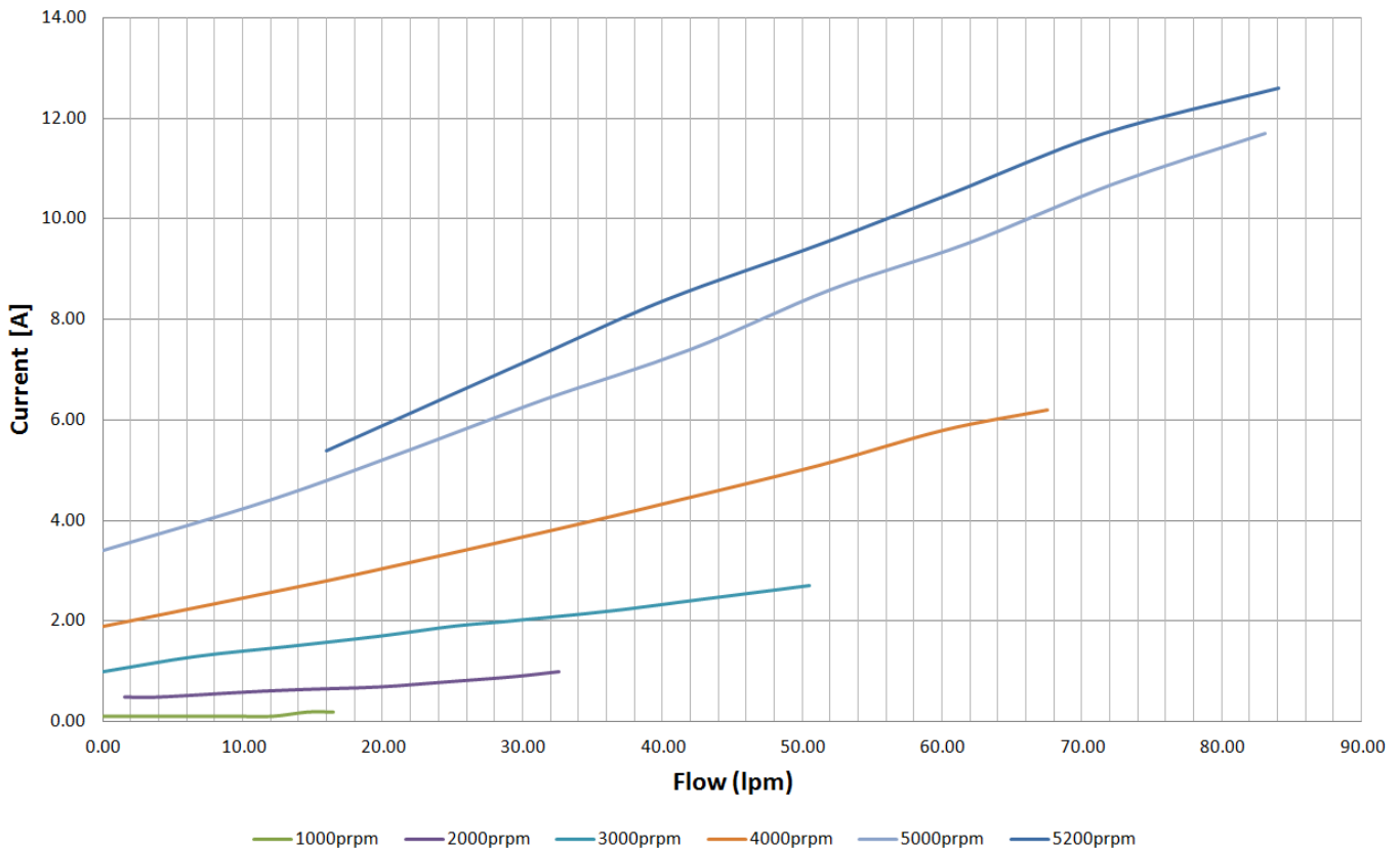
Current - 60°C 50/50 Water Glycol, 0.75Bar inletP
