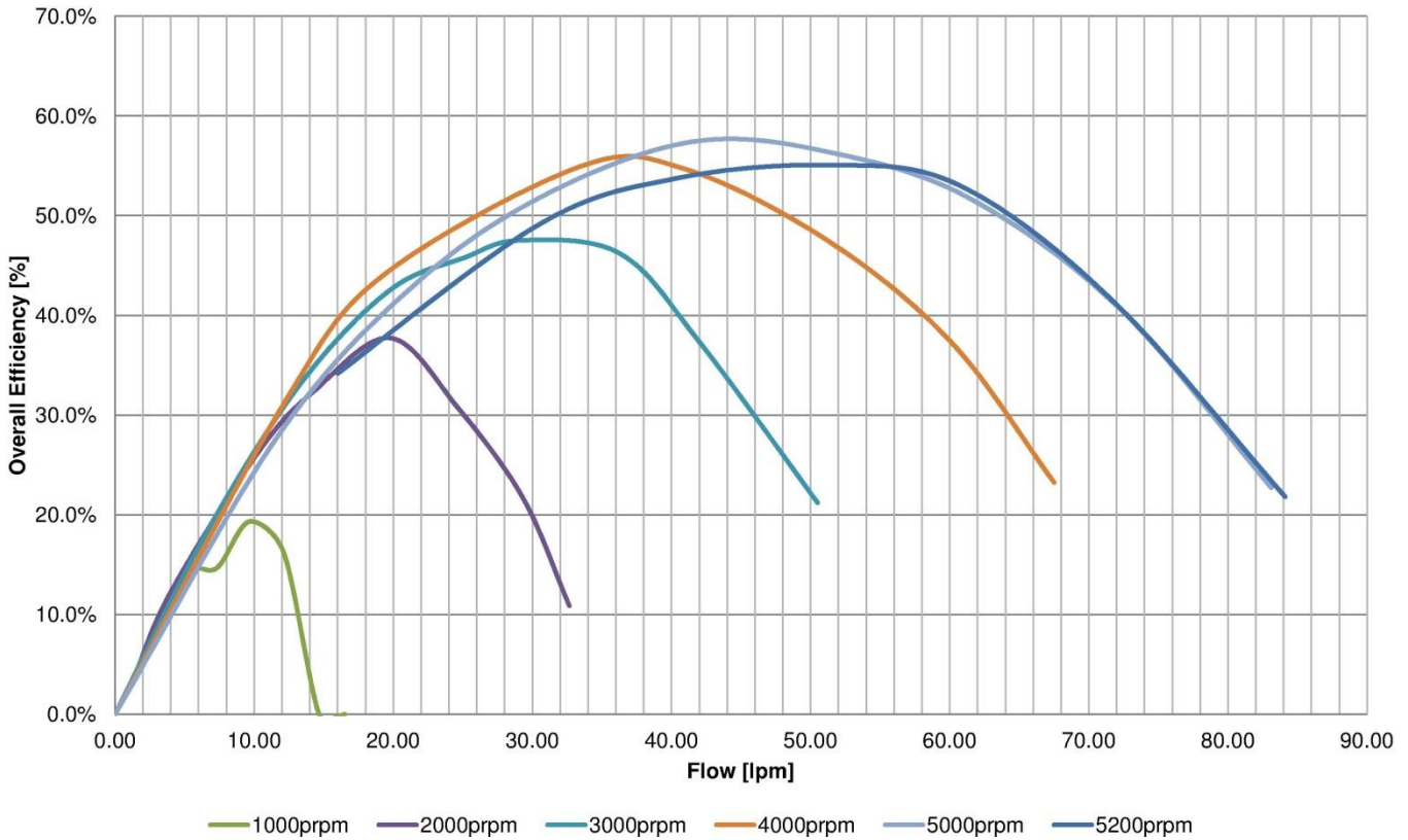
Efficiency flow curves - 60°C, 50/50 Water Glycol, 0.75bar inletP,
