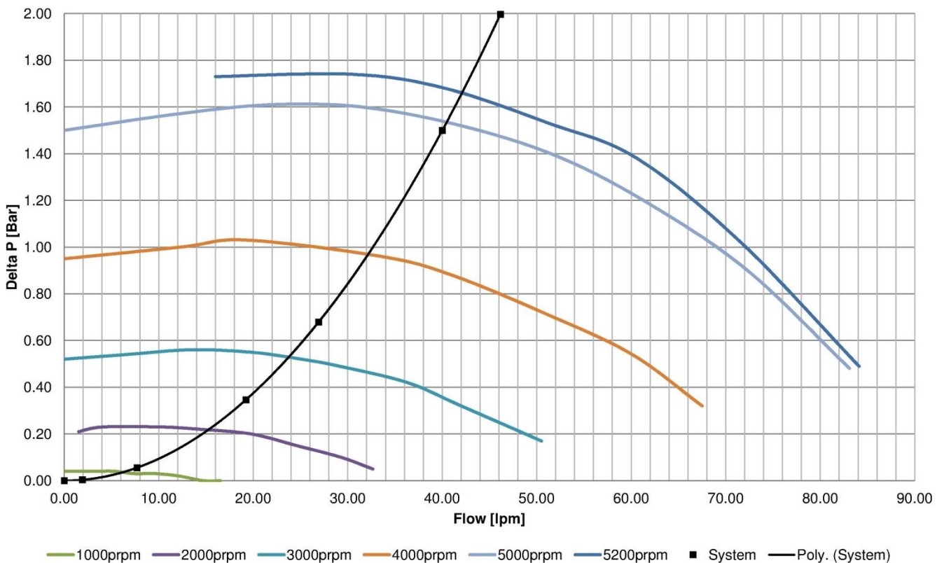
Performance curves - 60°C, 50/50 Water Glycol, 0.75bar inletP,
